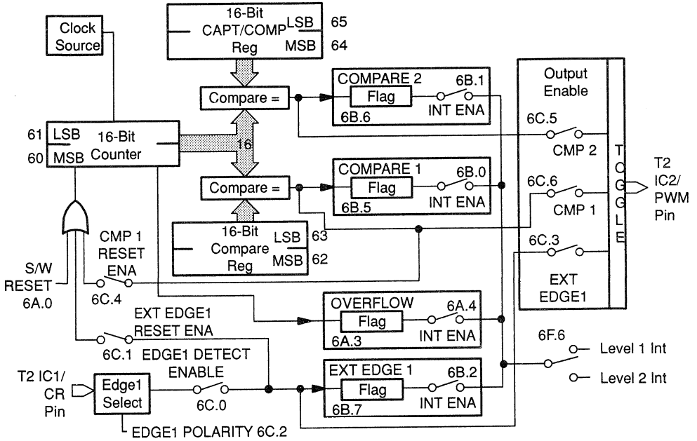
Figure B-7. Timer 2: Dual Compare Mode
