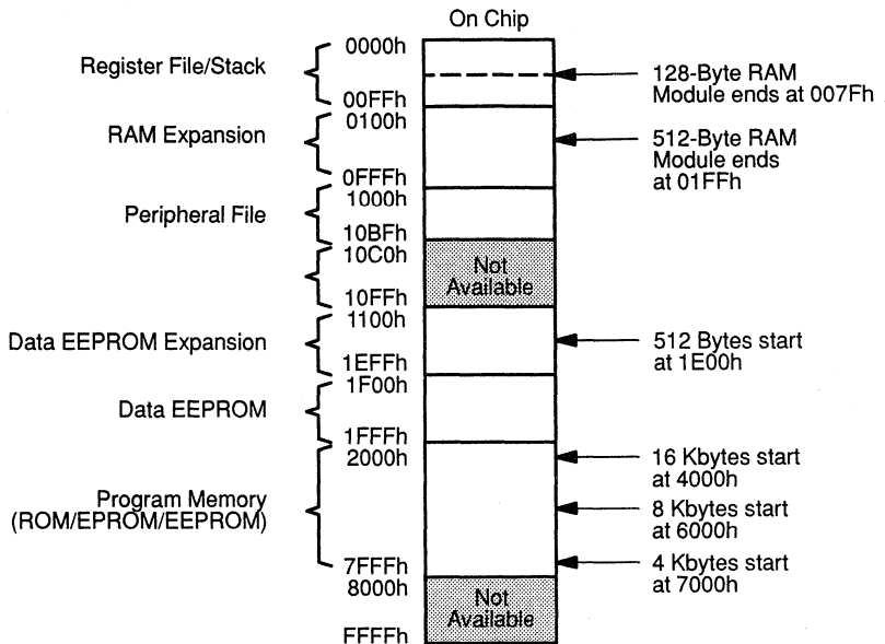
Figure 3–6. Microcomputer, Single Chip Mode
