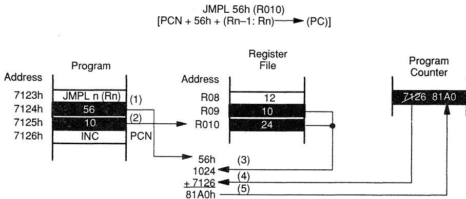
Figure 13–14. Relative Offset Indirect Addressing Mode
