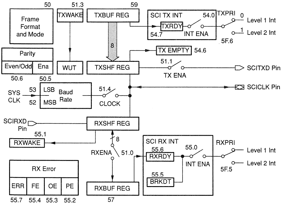
Figure B-9. SCI Block Diagram
