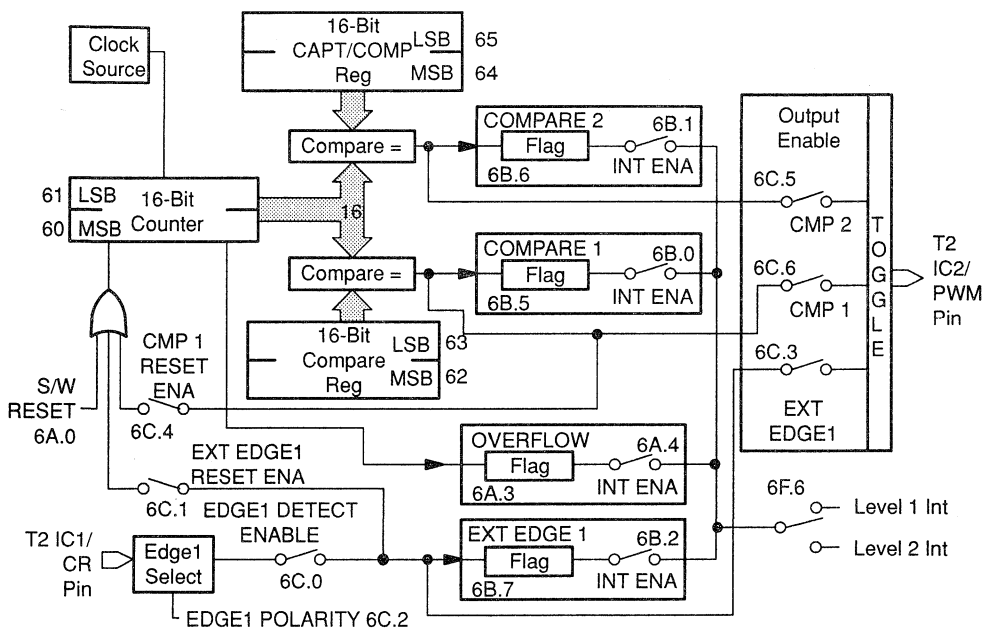
Figure 8–2. Dual Compare Mode
