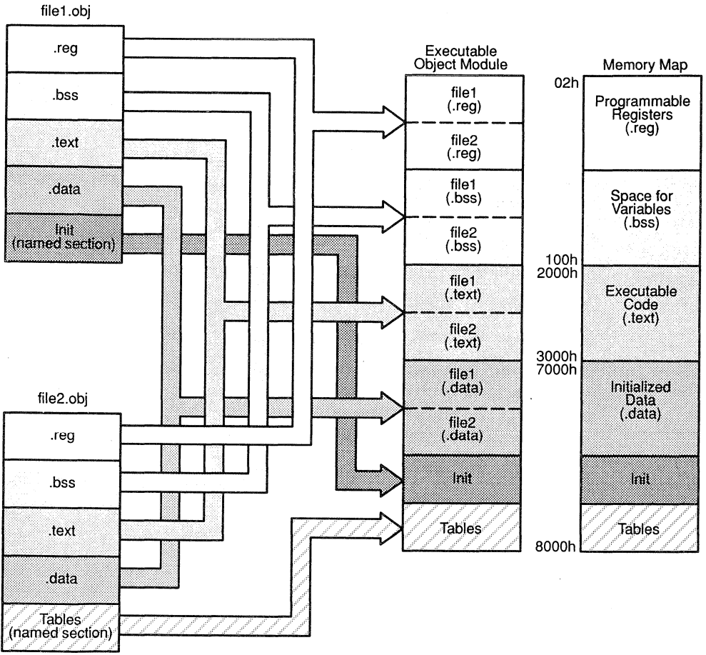
Figure 15-2. Linker Output Generation
