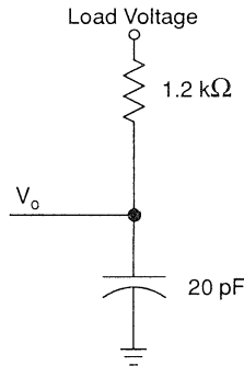
Figure 16–9. Typical Output Load Circuit §
