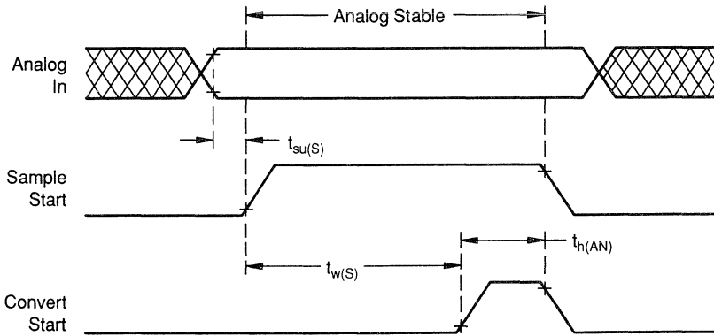
16 Figure 16–13. Analog Timing
