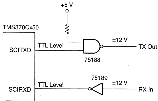
Figure 14–9. SCI/RS–232 Interface Example
