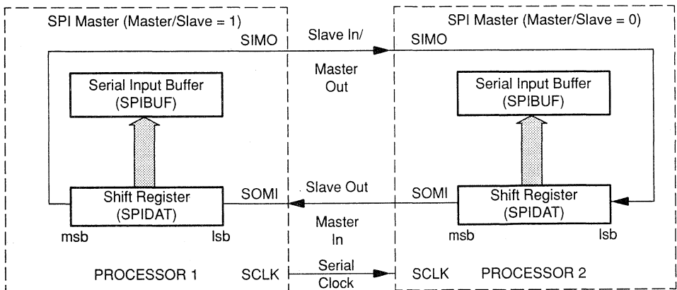
Figure 10–2. SPI Master/Slave Connection
