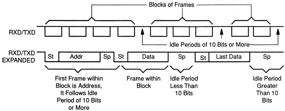
Figure 9–7. Idle Line Multiprocessor Communication Format
