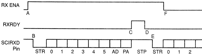
Figure 9–5. SCI RX Signals in Communication Modes
