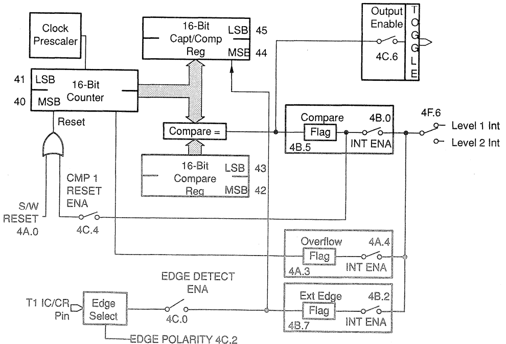
Figure 7-3. Capture/Compare Mode
