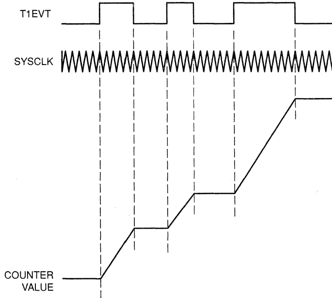
Figure 7–5. Pulse Accumulation
