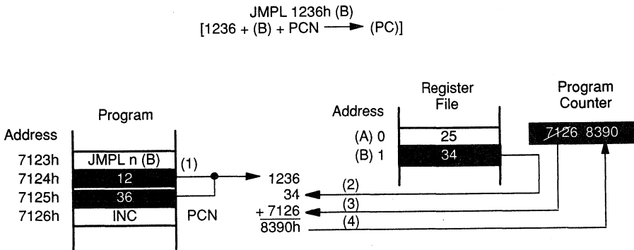
Figure 13–10. Relative Indexed Addressing Mode
