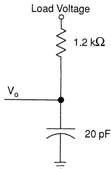
Figure 16–2. Typical Output Load Circuit §
