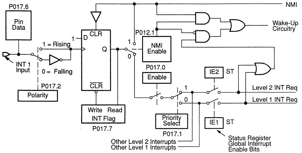
Figure 5-3. Interrupt 1 Block Diagram
