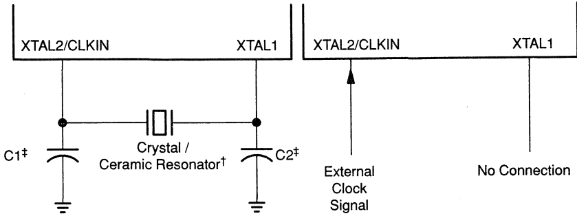
Figure 16–14. Recommended Crystal/Clock Connections
