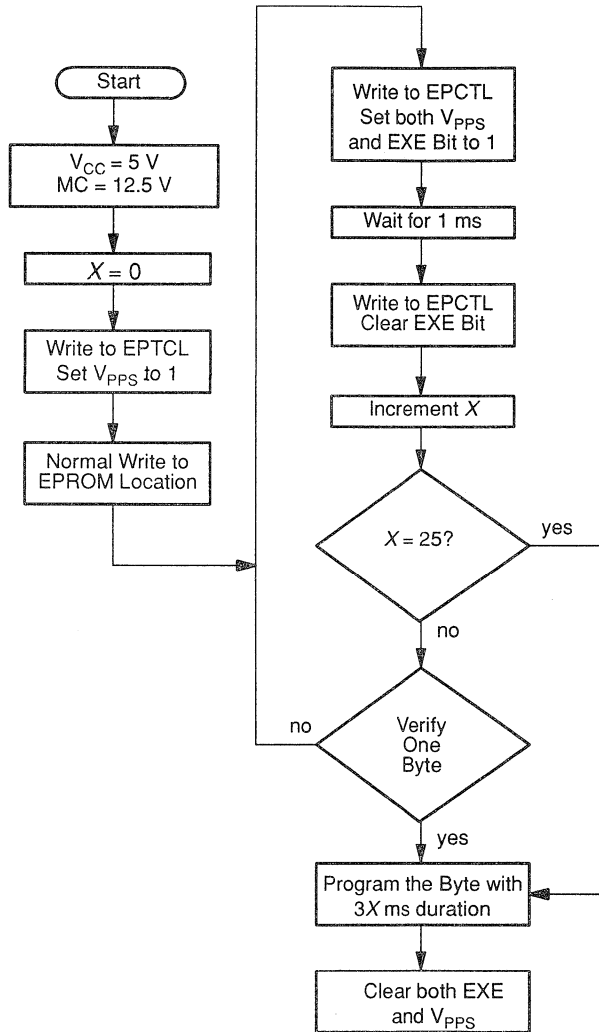
Figure 6-3. EPROM Programming Operation
