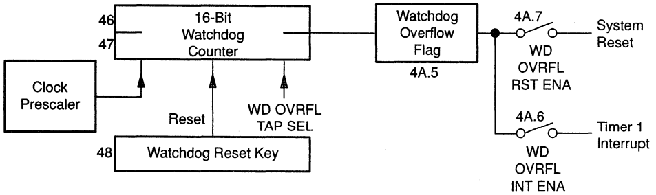
Figure B-4. Timer 1: Watchdog Timer
