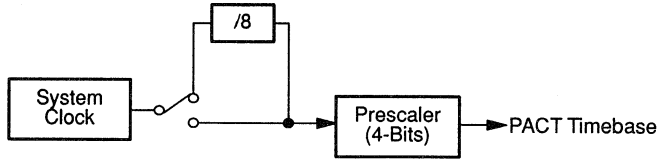
Figure 12–10. Prescaler Circuit
