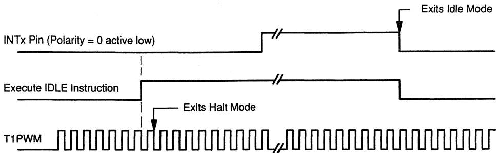
Figure 4–3. Improper Method to Enter Halt Mode
