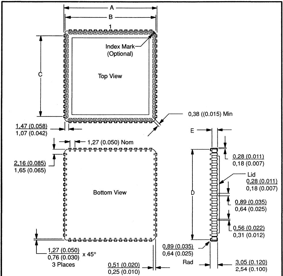
Figure 17-4. Ceramic Leaded Chip Carrier Package (FJ Suffix)
