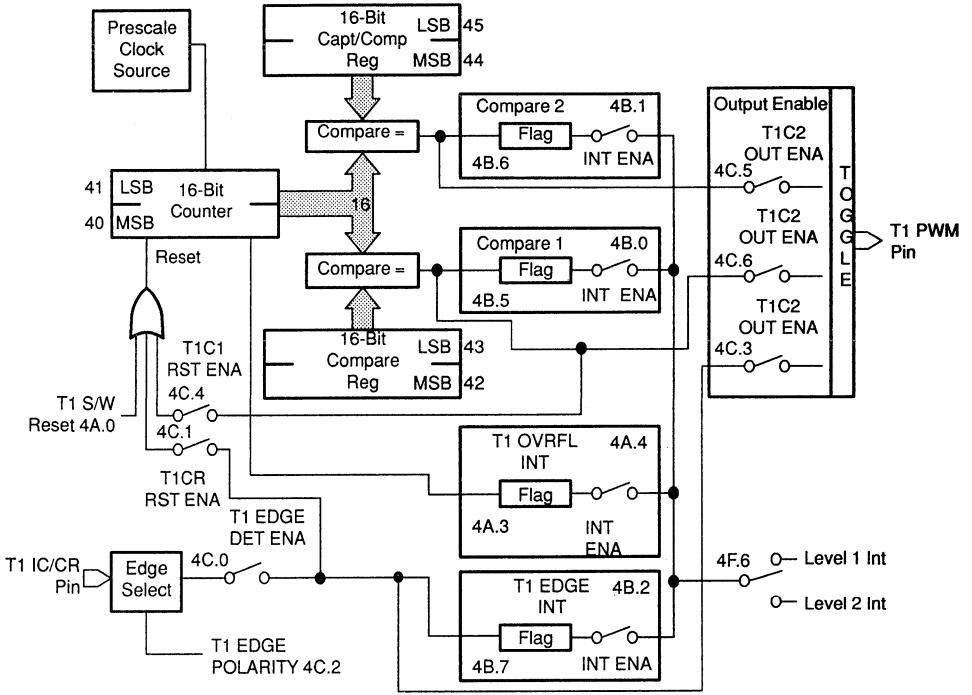
Figure B-5. Timer 1: Dual Compare Mode
