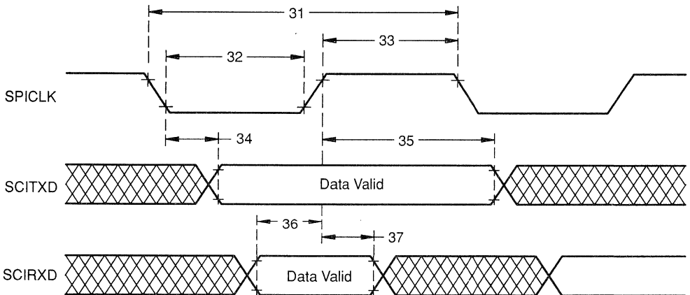
Figure 16–23. SCI Isosynchronous Mode Timing Diagram for External Clock
