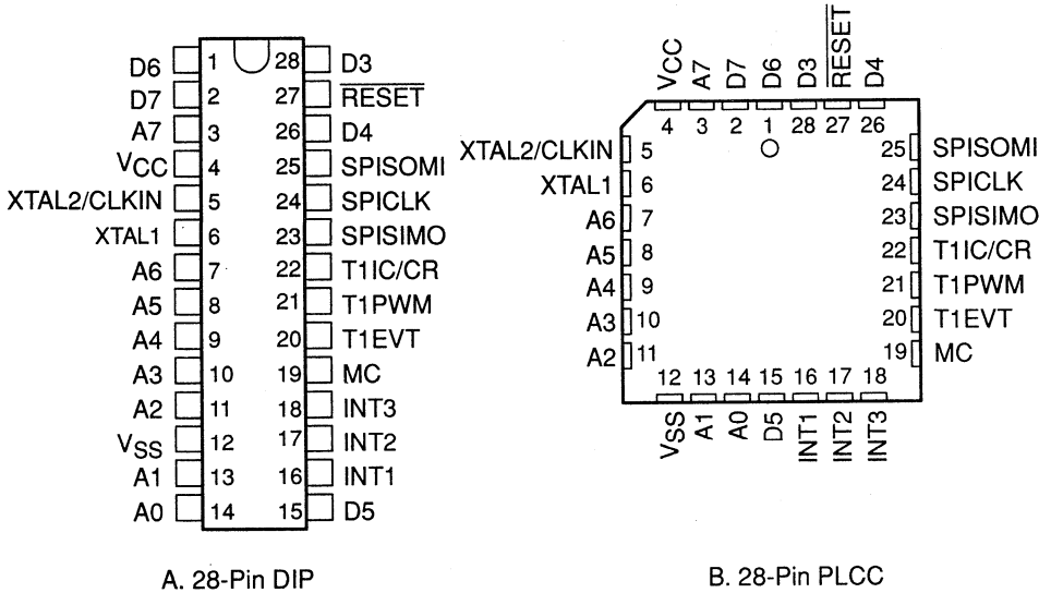
Figure 2–1. Pinouts for TMS370Cx1x
