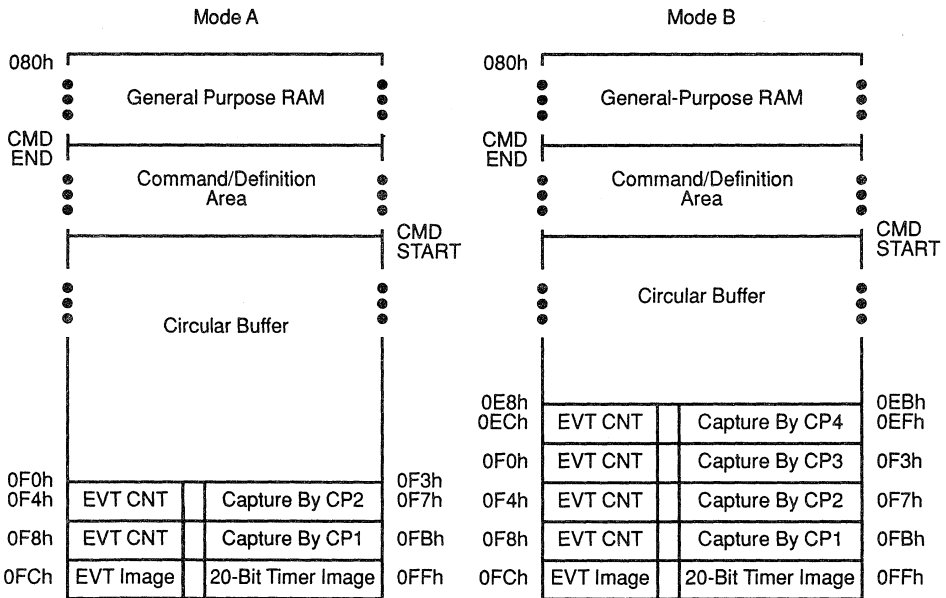
Figure 12–4. Dual-Port RAM Organization
