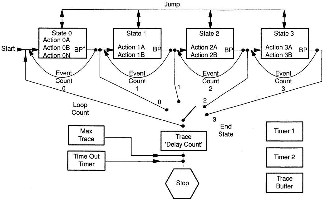
Figure 15-5. BTT Operation (XDS/22 Systems Only)
