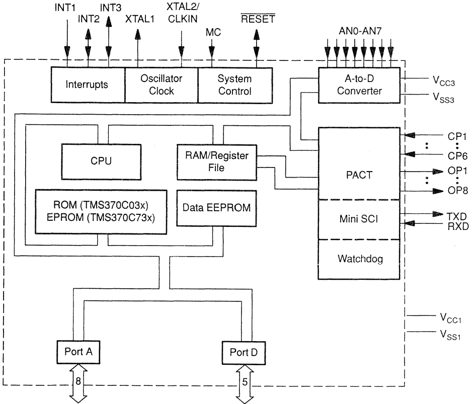
Figure 1–2. TMS370Cx3x Block Diagram
