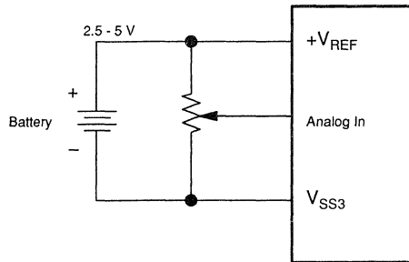
Figure 11–2. Ratiometric Conversion Example
