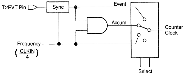
Figure 8–4. Timer 2 Clock Sources
