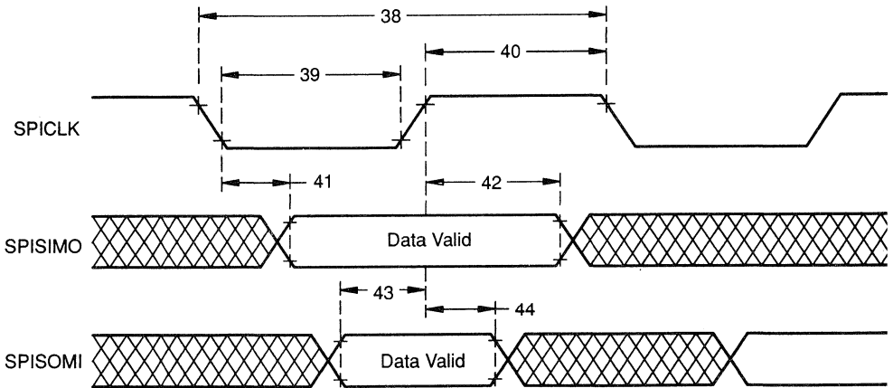
Figure 16–20. SPI Master External Timing
