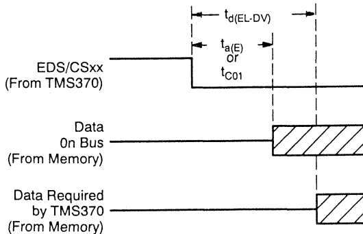
Figure 14-3. Chip Select Low To Data Read Timing
