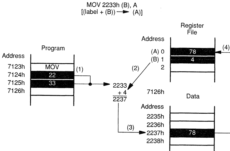
Figure 13–9. Absolute Indexed Addressing Mode
