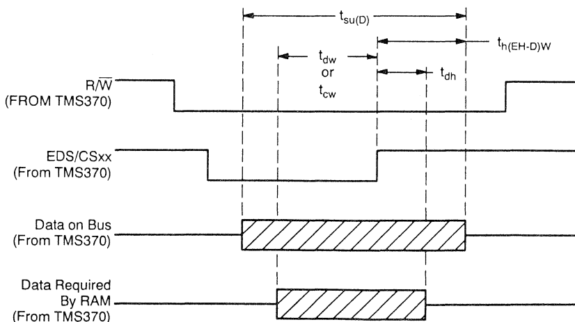
Figure 14–6. Write Data Setup Timing
