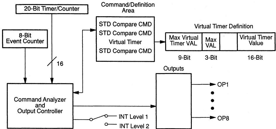
Figure 12-8. Virtual Timer Implementation
