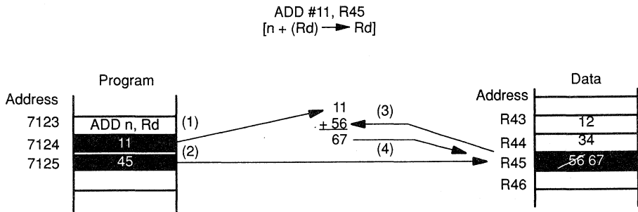
Figure 13–4. Immediate Addressing Mode
