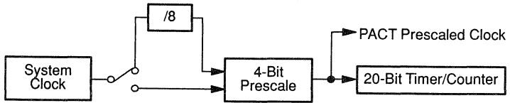
Figure 12–2. Time Base Block Diagram
