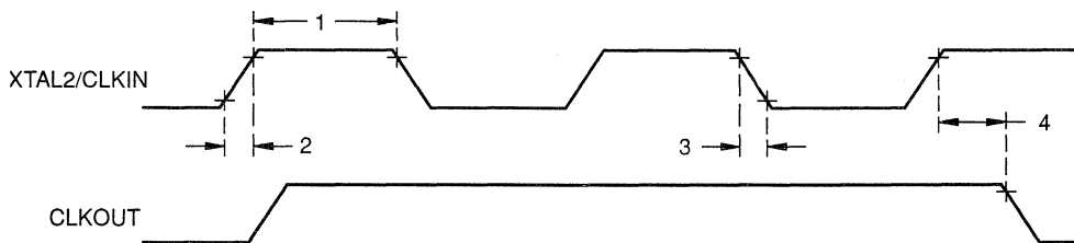
Figure 16–3. External Clock Timing
