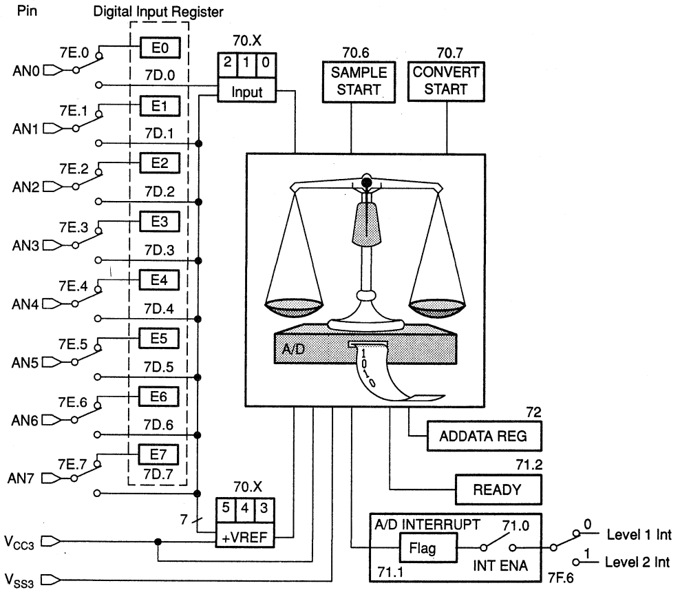
Figure 11–1. Analog-to-Digital Converter Block Diagram
