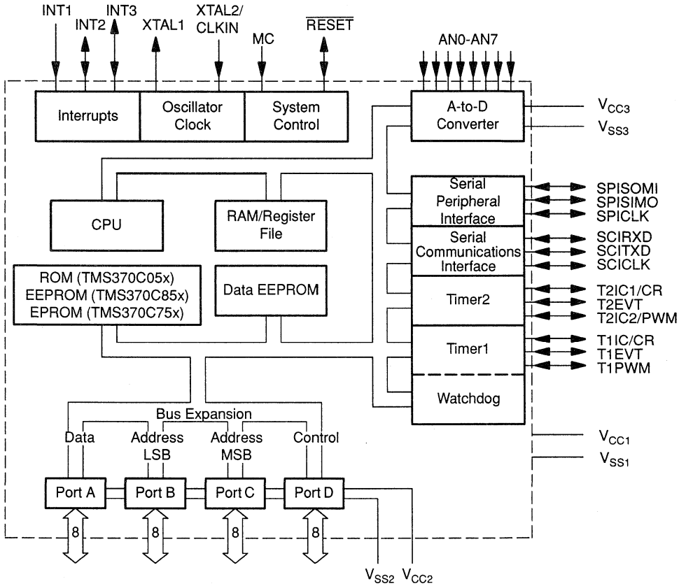
Figure 1–3. TMS370Cx5x Block Diagram
