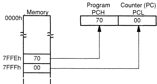
Figure 3–3. Program Counter After Reset
