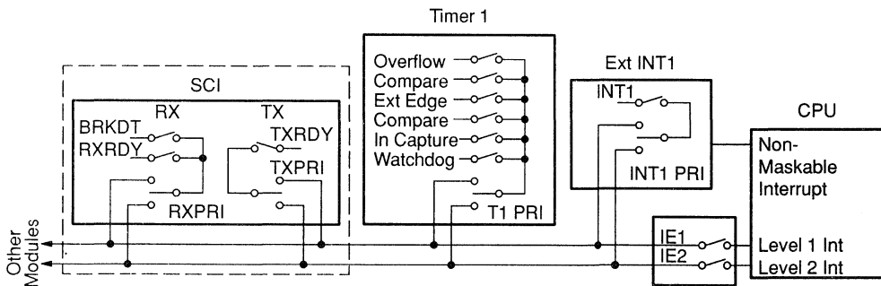
Figure 5–1. Interrupt Control
