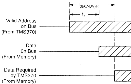
Figure 14–2. Valid Address-To-Data Read Timing
