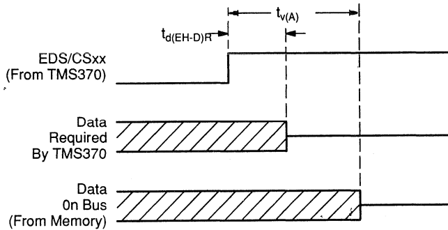
Figure 14-5. Read Data Hold After Chip Select High Timing
