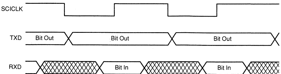
Figure 9–4. Isosynchronous Communication Format
