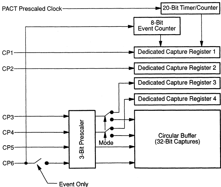
Figure 12–3. Input Capture Block Diagram
