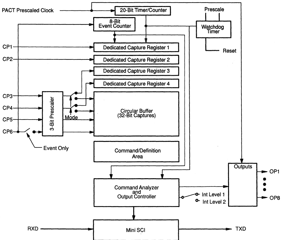
Figure 12–11. PACT Block Diagram
