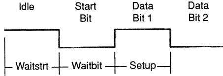
14 Figure 14–10. Auto Baud Rate Waveform
