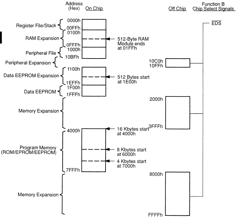
Figure 3–8. Microcomputer Mode with Function B Expansion
