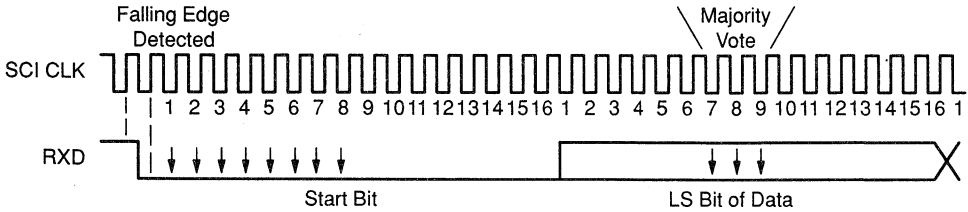
Figure 9–3. Asynchronous Communication Format
