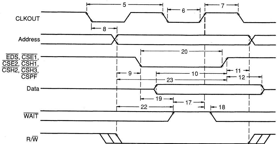
Figure 16–19. External Write Timing
