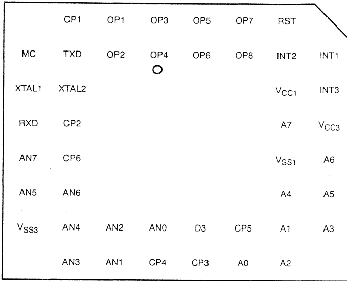
Figure F-4. TMS370Cx3x Device PGA Pinout (Bottom View)
