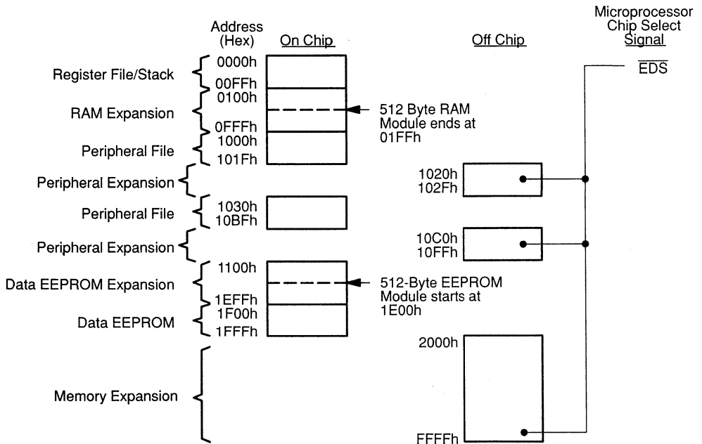
Figure 3–9. Microprocessor Mode without Internal Memory
