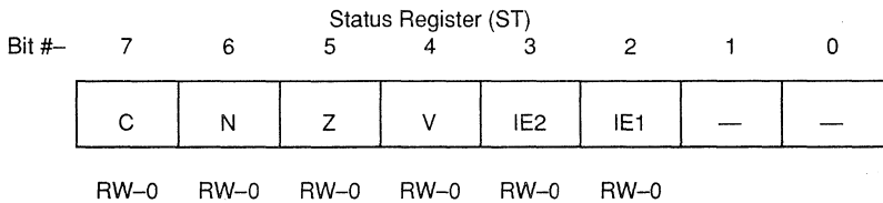
Figure 13–15. Status Register (ST)
