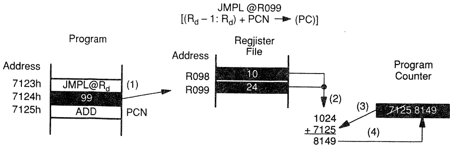
Figure 13–12. Relative Indirect Addressing Mode
