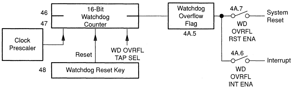
Figure 7–6. Watchdog Timer
