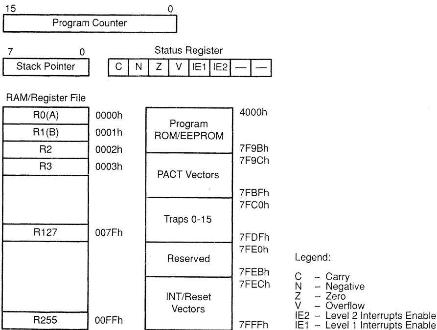
Figure 3–1. Programmer’s Model
