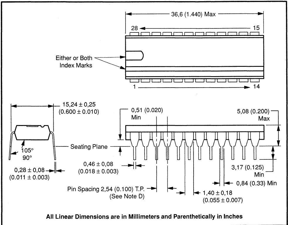
Figure 17-2. 28-Pin Plastic Dual-Inline Package, 100-MIL Pin Spacing (Type N Package Suffix)
