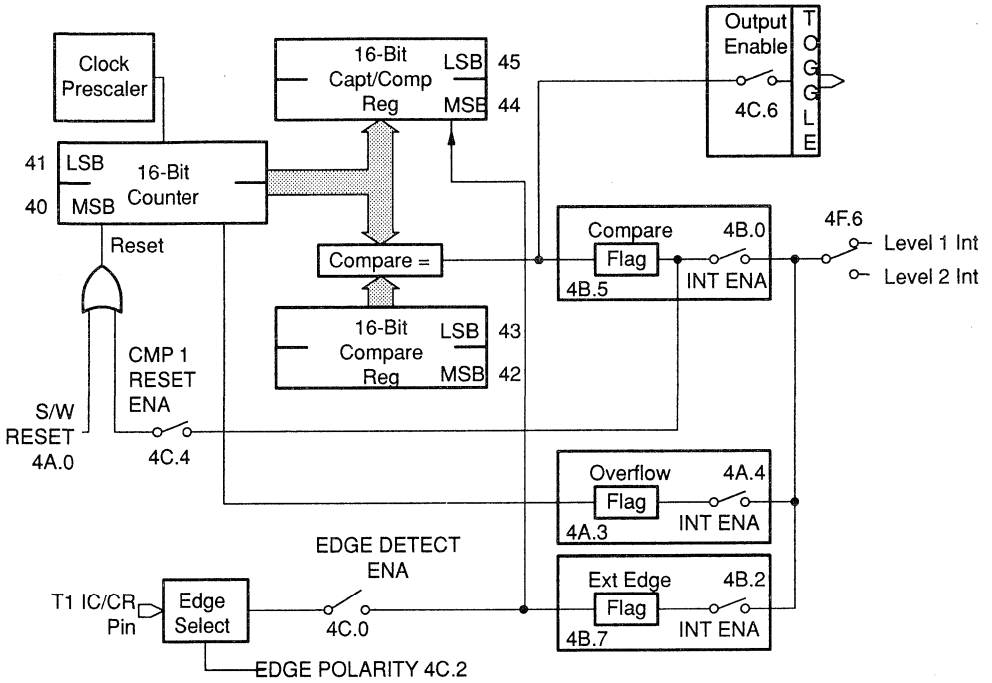
Figure B-6. Timer 1: Capture/Compare Mode
