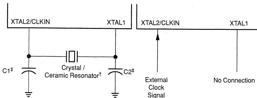
Figure 16–1. Recommended Crystal/Clock Connections
