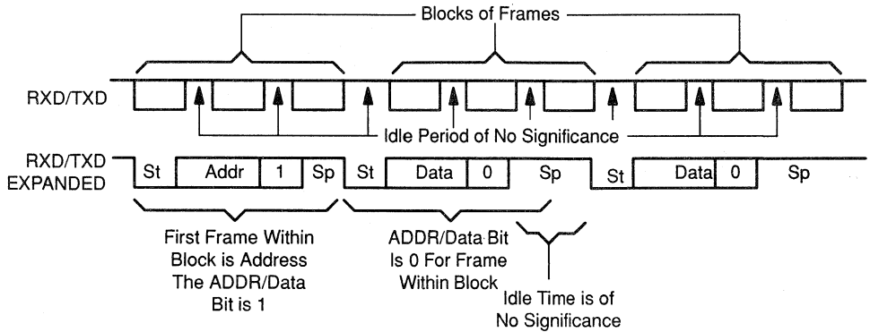
Figure 9–9. Address Bit Multiprocessor Communication Format
