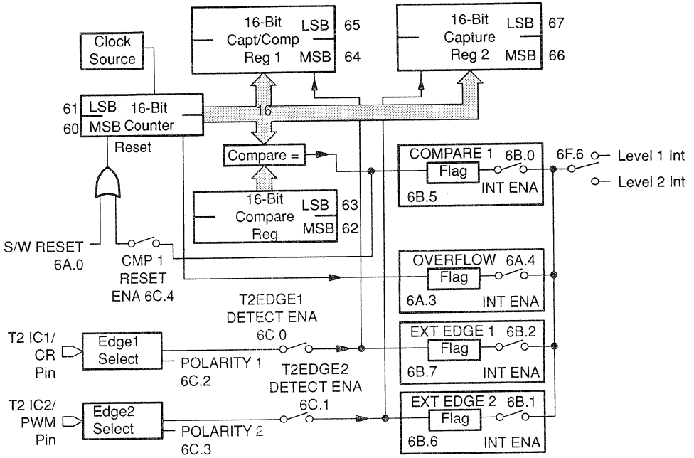
Figure B-8. Timer 2: Dual Capture Mode
