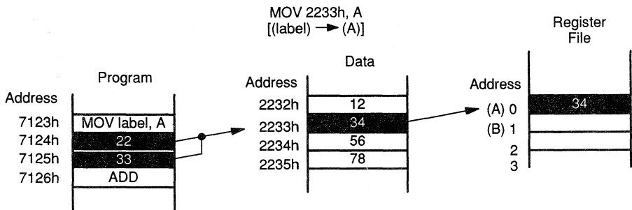
Figure 13–7. Absolute Direct Addressing Mode
