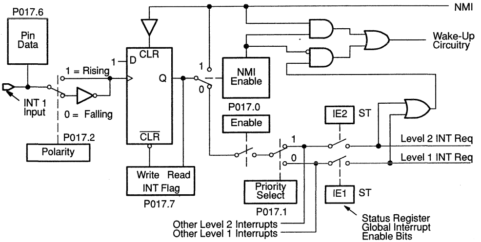
Figure B-1. Interrupt 1 Block Diagram
