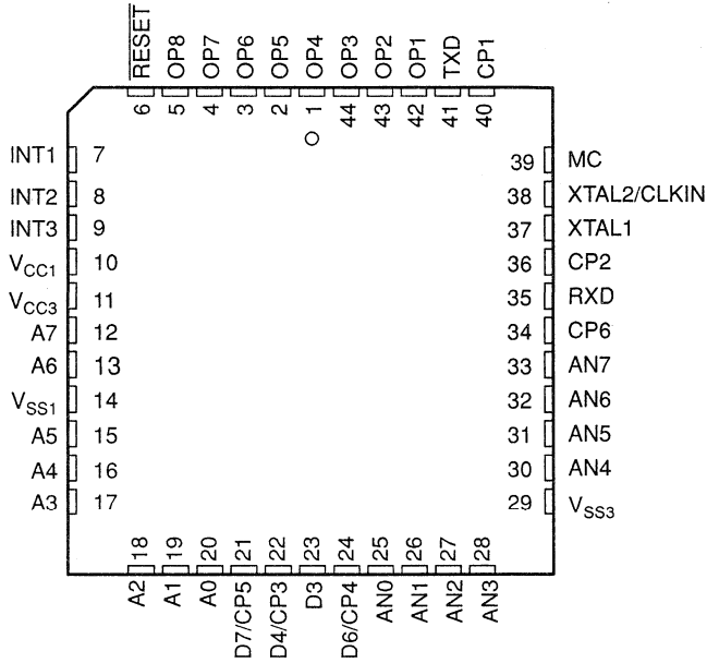
Figure 2–2. Pinout for TMS370Cx3x
