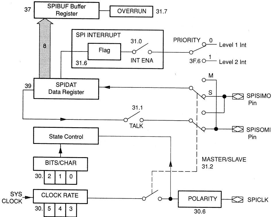
Figure 10–1. SPI Block Diagram
