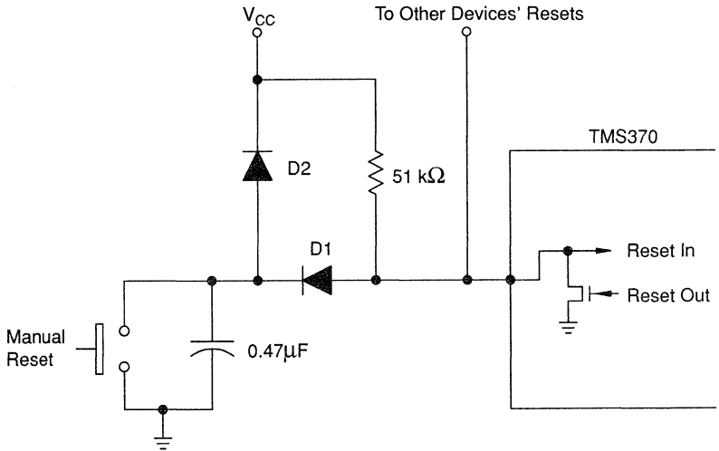
Figure 5–5. Typical Reset Circuit
