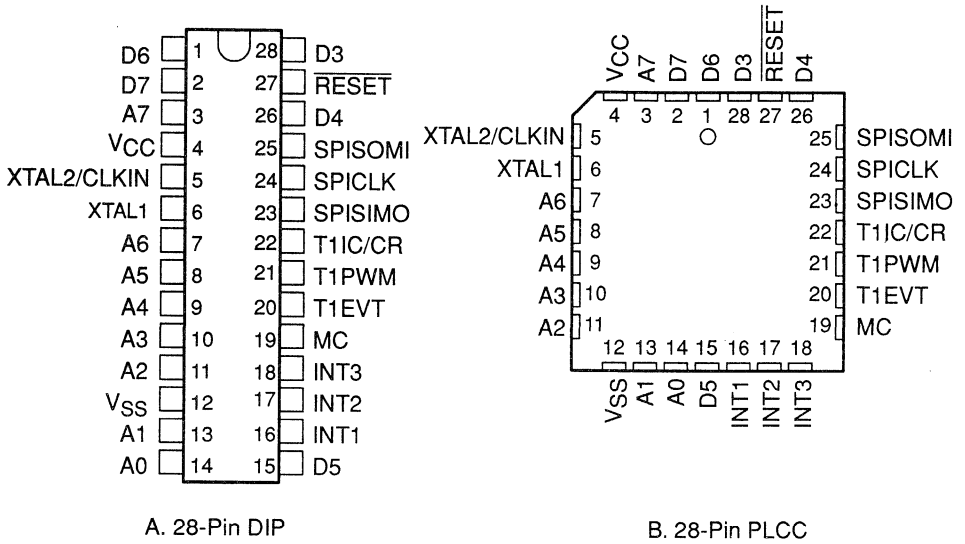
Figure F-7. Pinouts for TMS370Cx1x (Top View)
