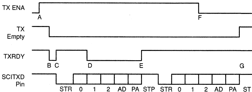
Figure 9–6. SCI TX Signals in Communications Modes
