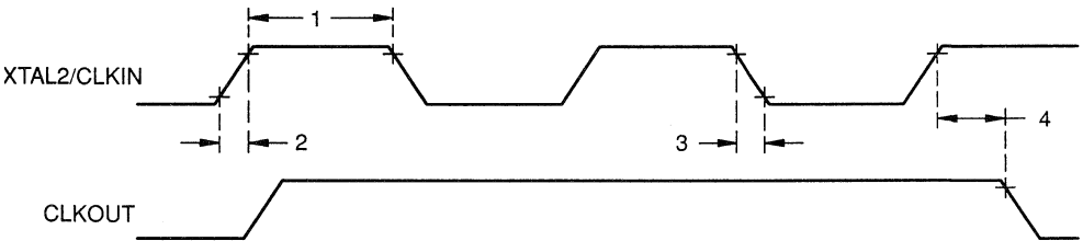
Figure 16–16. External Clock Timing
