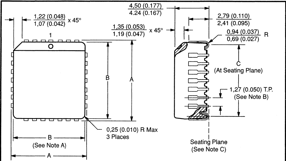
Figure 17-3. Plastic-Leaded Chip Carrier Package (Type FN Package Suffix)
