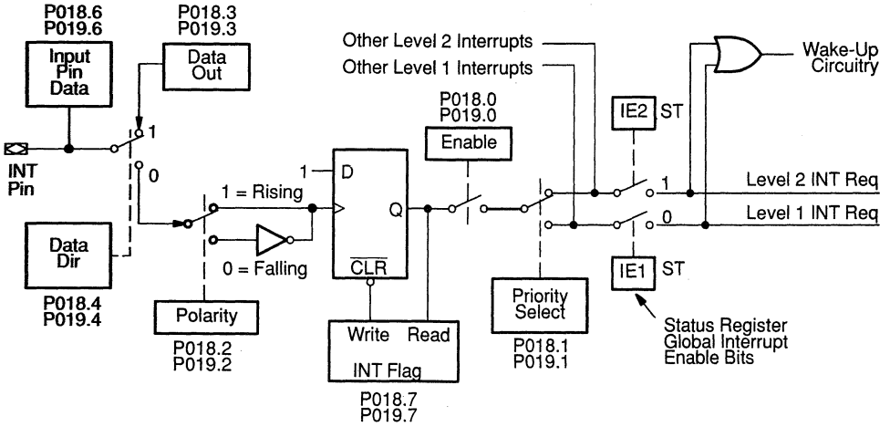
Figure B-2. Interrupts 2 and 3 Block Diagram
