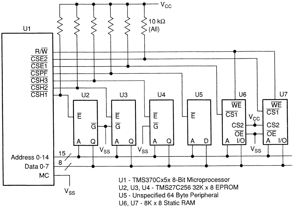
Figure 14-1. Microcomputer Interface Example
