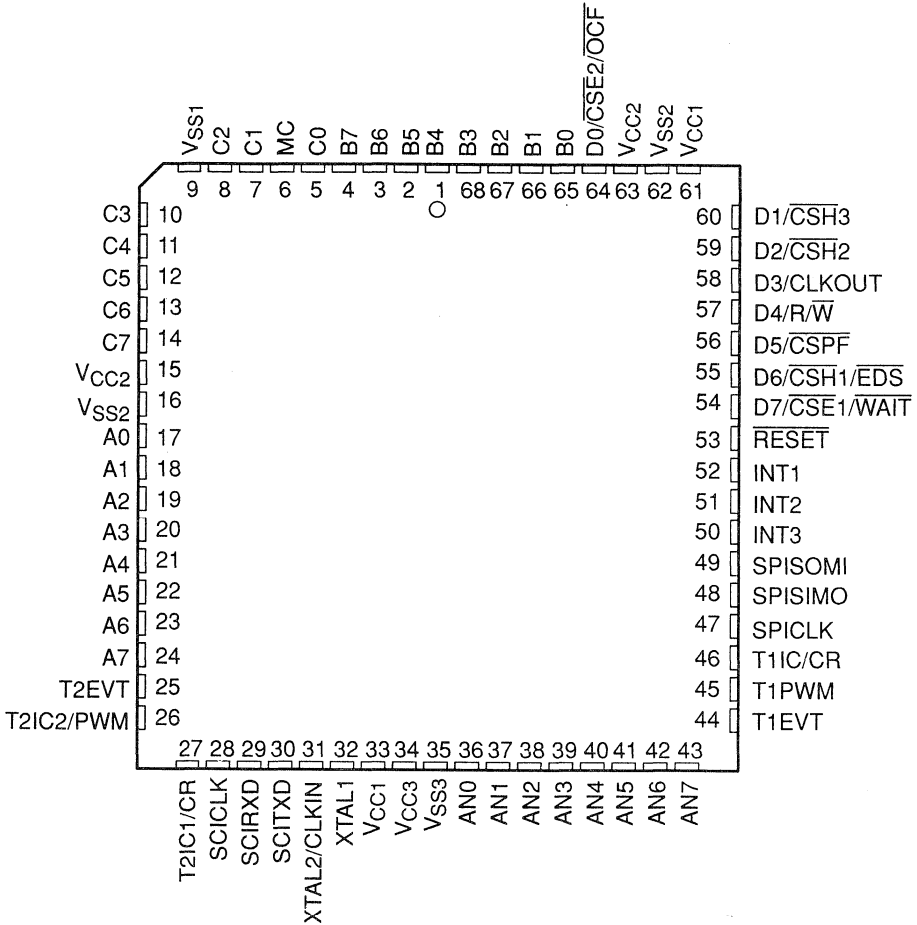
2 Figure 2–3. Pinouts for TMS370Cx5x
