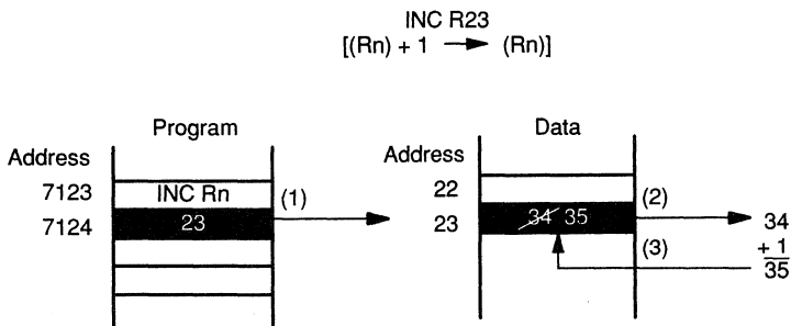
Figure 13–2. Register Addressing Mode
