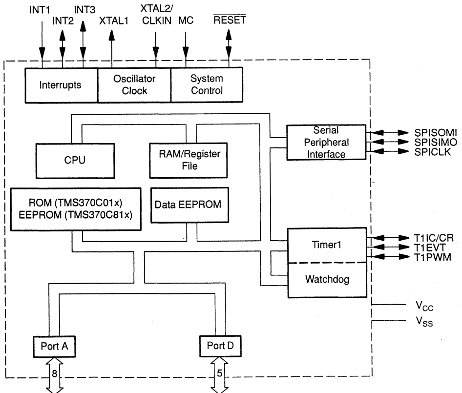
Figure 1-1. TMS370Cx1x Block Diagram
