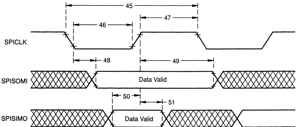
Figure 16–21. SPI Slave External Timing
