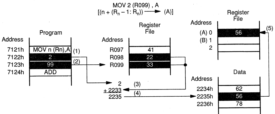
Figure 13–13. Absolute Offset Indirect Addressing Mode
