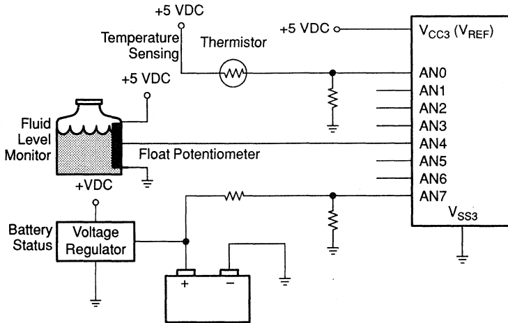
Figure 14–11. A/D Converter Sample Applications
