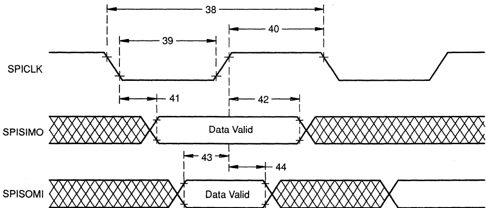
Figure 16–6. SPI Master External Timing
