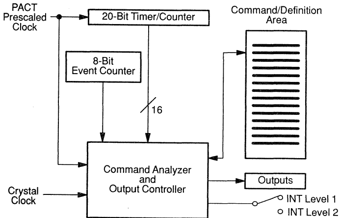
Figure 12–6. Output Control Section
