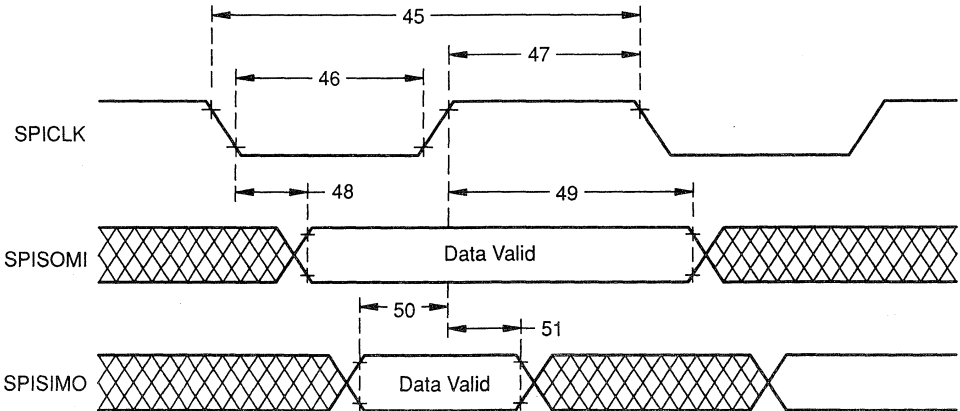
Figure 16–7. SPI Slave External Timing
