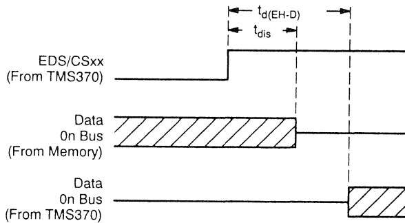
Figure 14-4. Chip Select High To Next Data Bus Drive Timing
