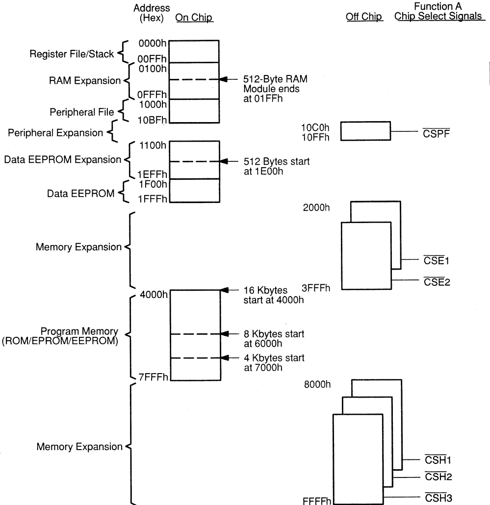
Figure 3–7. Microcomputer Mode with Function A Expansion
