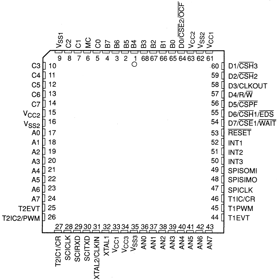
Figure F-9. Pinouts for TMS370Cx5x (Top View)
