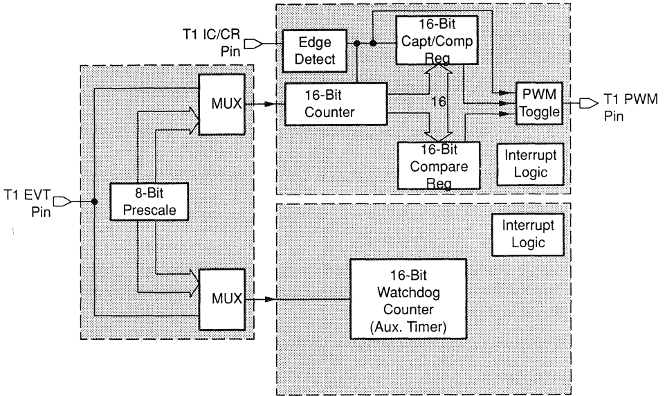
Figure 7–1. Timer 1 Block Diagram
