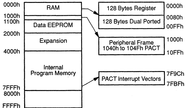
Figure 12-5. RAM Organization
