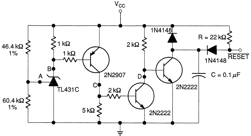
Figure 5–6. Typical Reset Circuit with Low-voltage Detection
