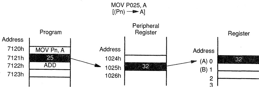
Figure 13–3. Peripheral Addressing Mode
